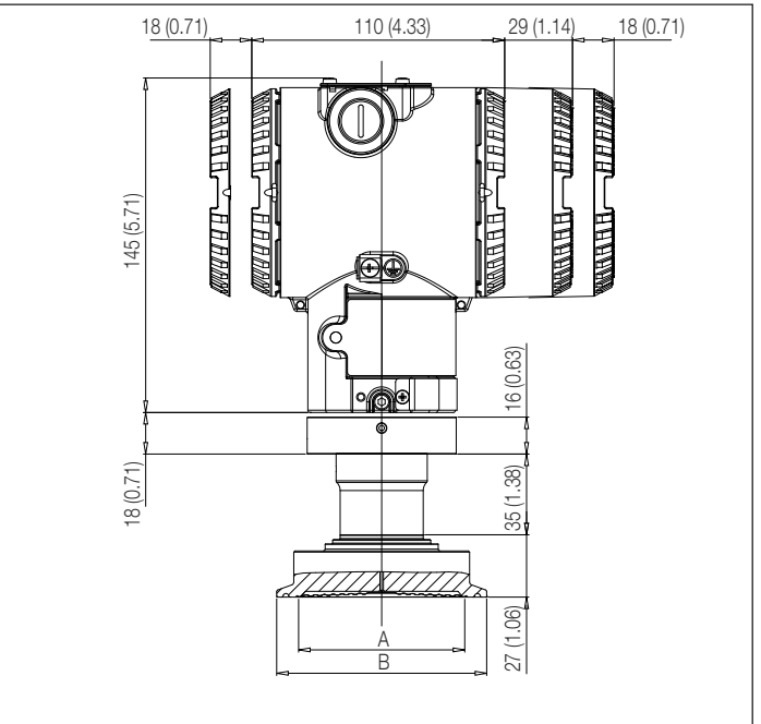
266HDH / 266NDH with barrel housing and direct mount seal S26SS Triclamp
