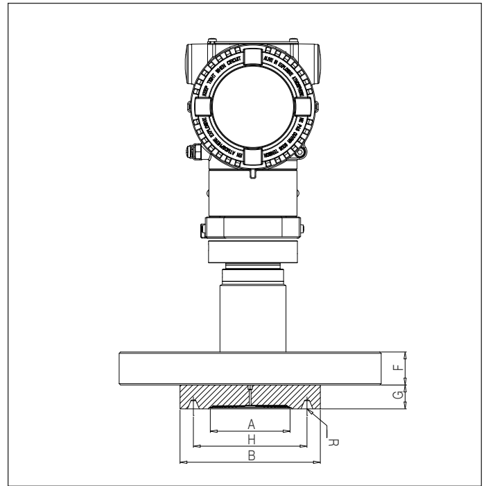
266HDH / 266NDH with barrel housing and direct mount seal S26RR flanged Ring Joint flush diaphragm
