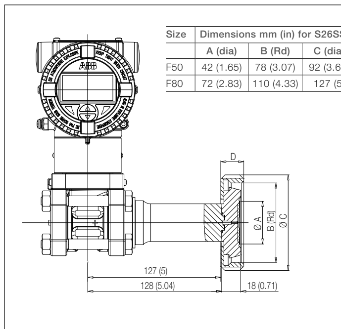
266DDH with barrel housing and direct mount seal S26SS Union Nut
