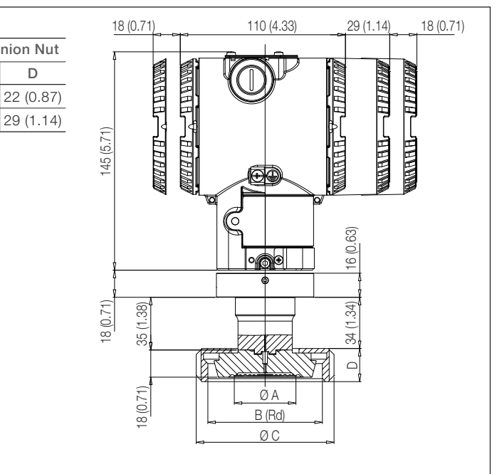
266HDH / 266NDH with barrel housing and direct mount seal S26SS Union Nut
