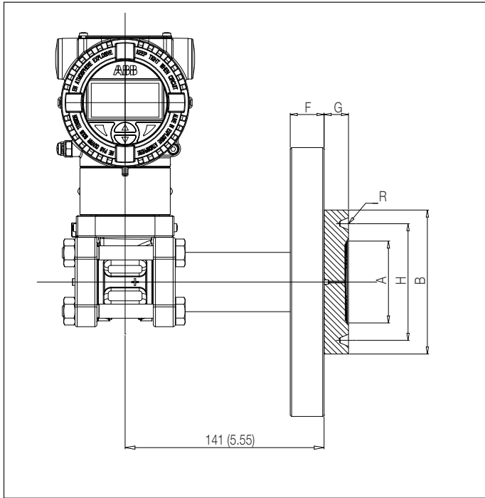
266DDH with barrel housing and direct mount seal S26RR flanged Ring Joint flush diaphragm
